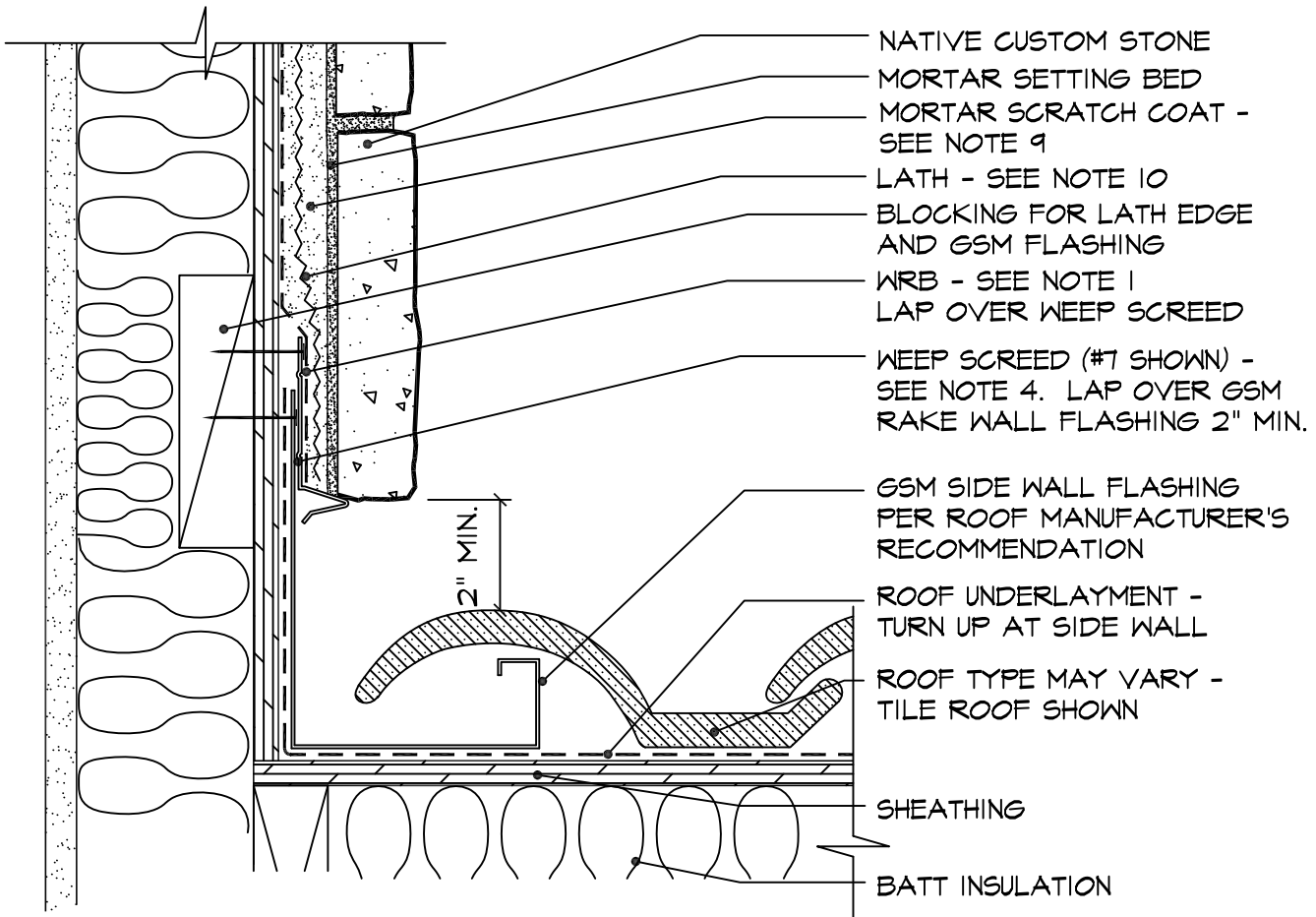
○ STONE AND FLASHING AT TILE ROOF SCALE: 3"=1'-0"
