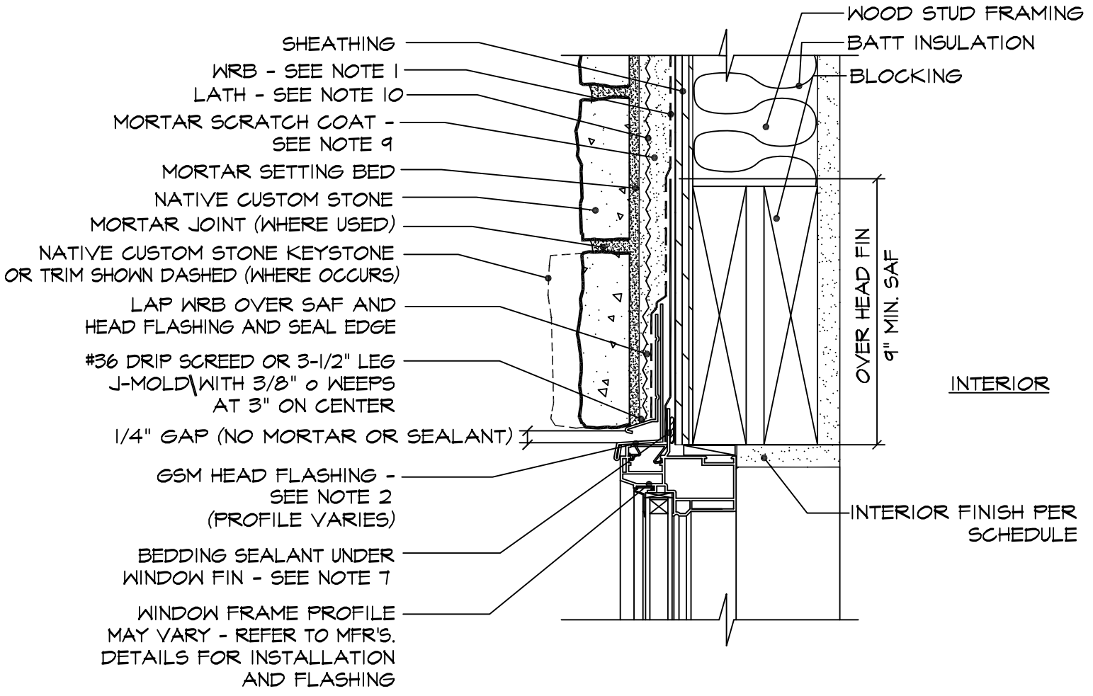
○ STONE @ WINDOW HEAD SCALE: 3"=1'-0"
