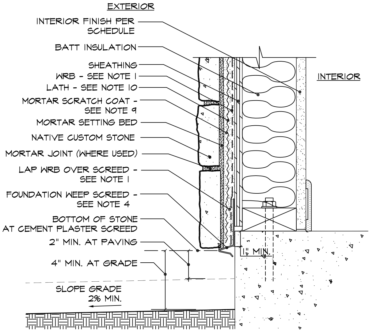
○ STONE @ WOOD FRAME/ CONC. FOUNDATION SCALE: 3"=1'-0"
