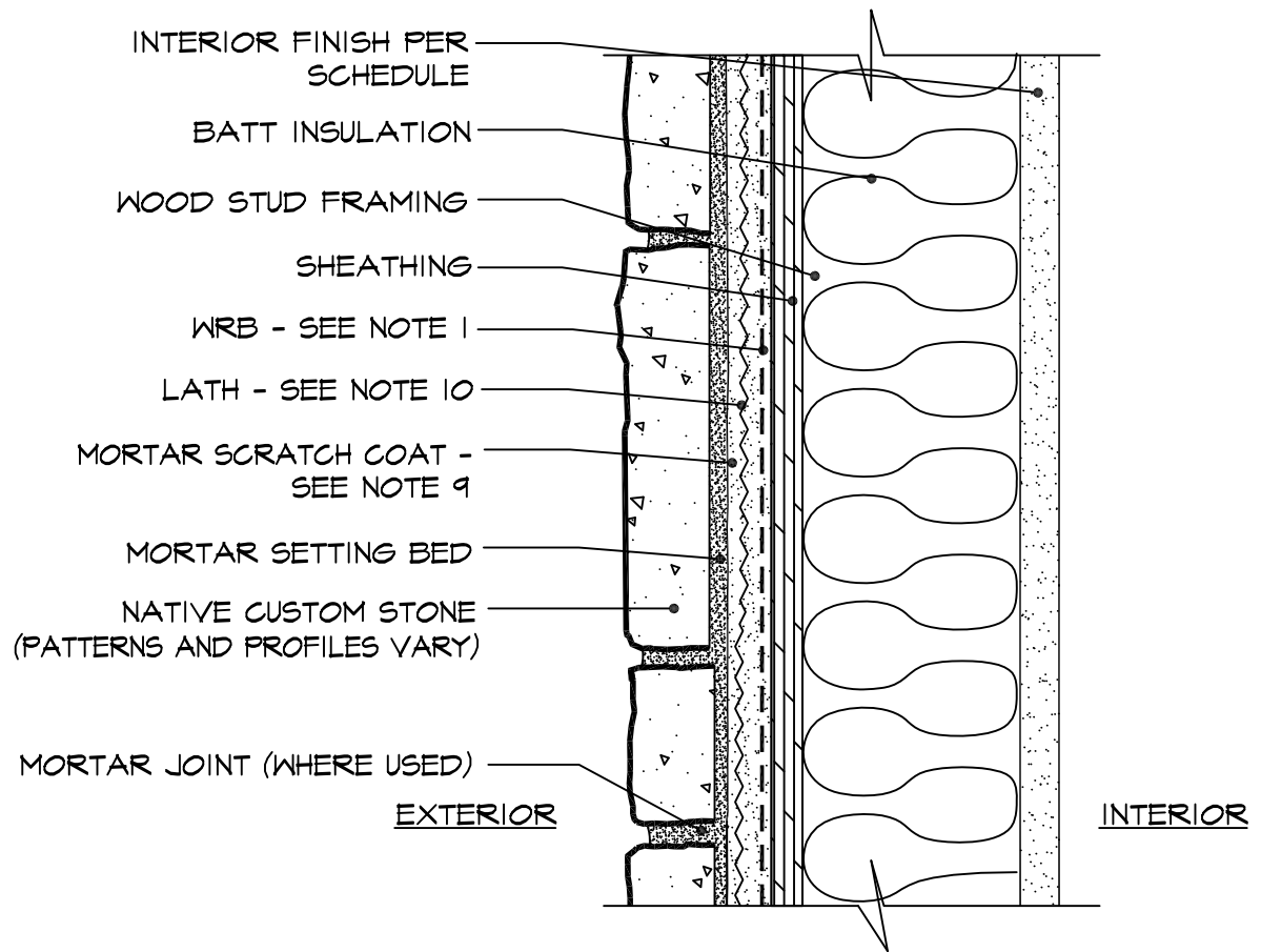
○ STONE @ WOOD FRAME - TYPICAL SCALE: 3"=1'-0"
