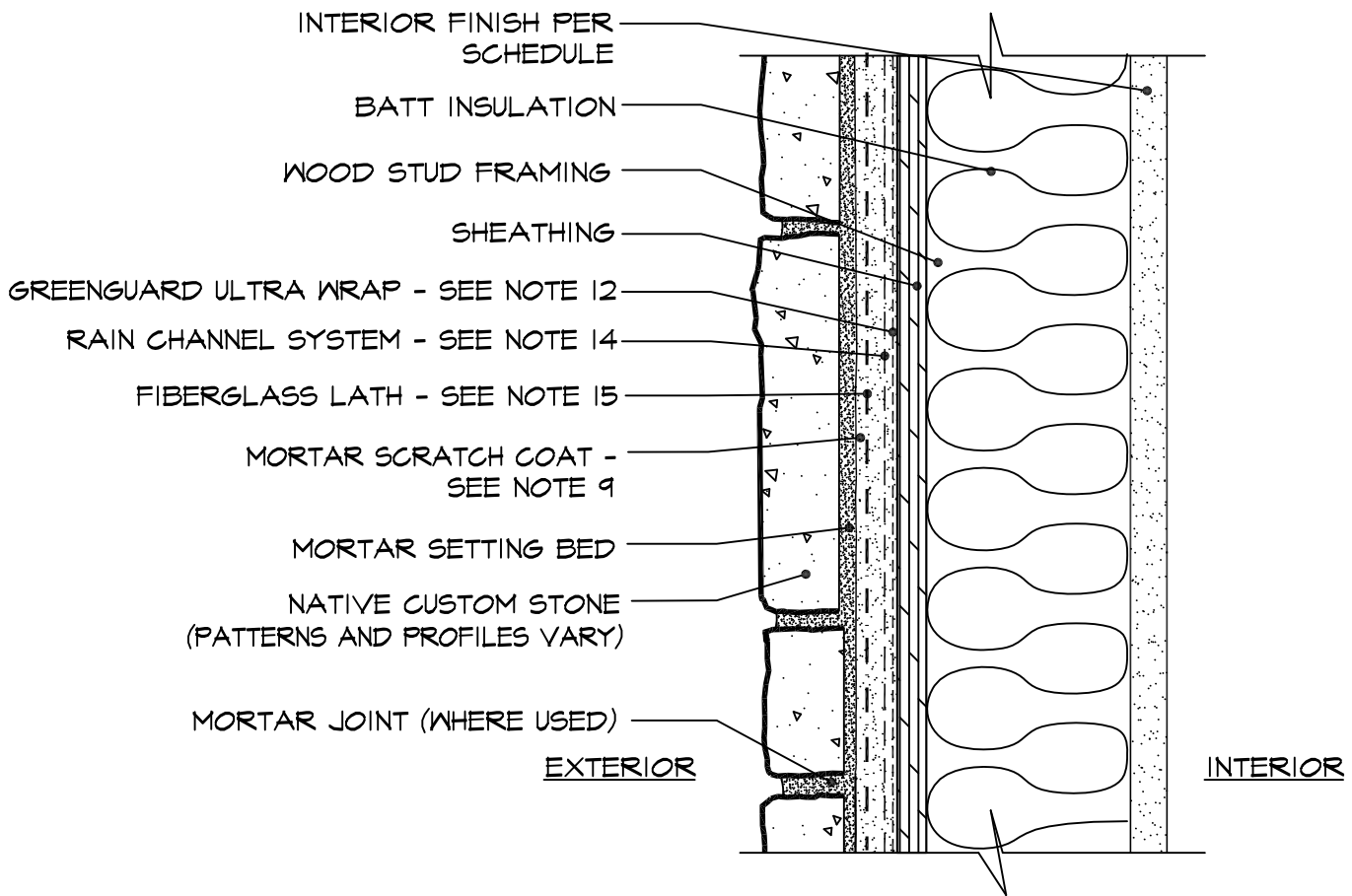
○ STONE @ WOOD FRAME - ALT. WATER PROTECTION SCALE: 3"=1'-0"
