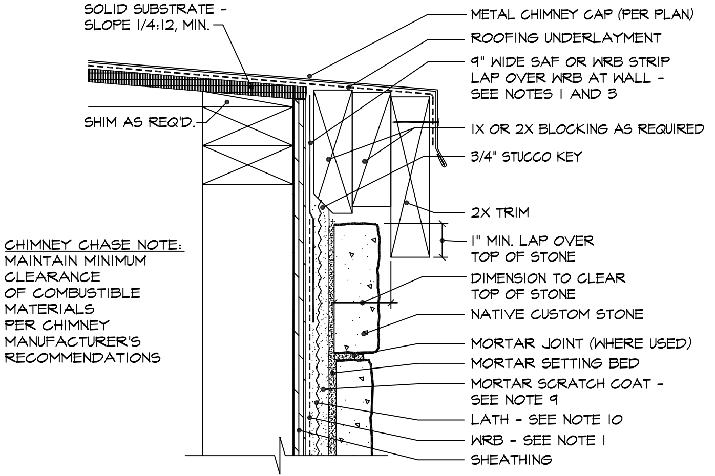
○ CHIMNEY CHASE CAP WITH WOOD TRIM SCALE: 3"=1'-0"
